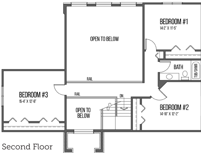
Optional Second Floor
